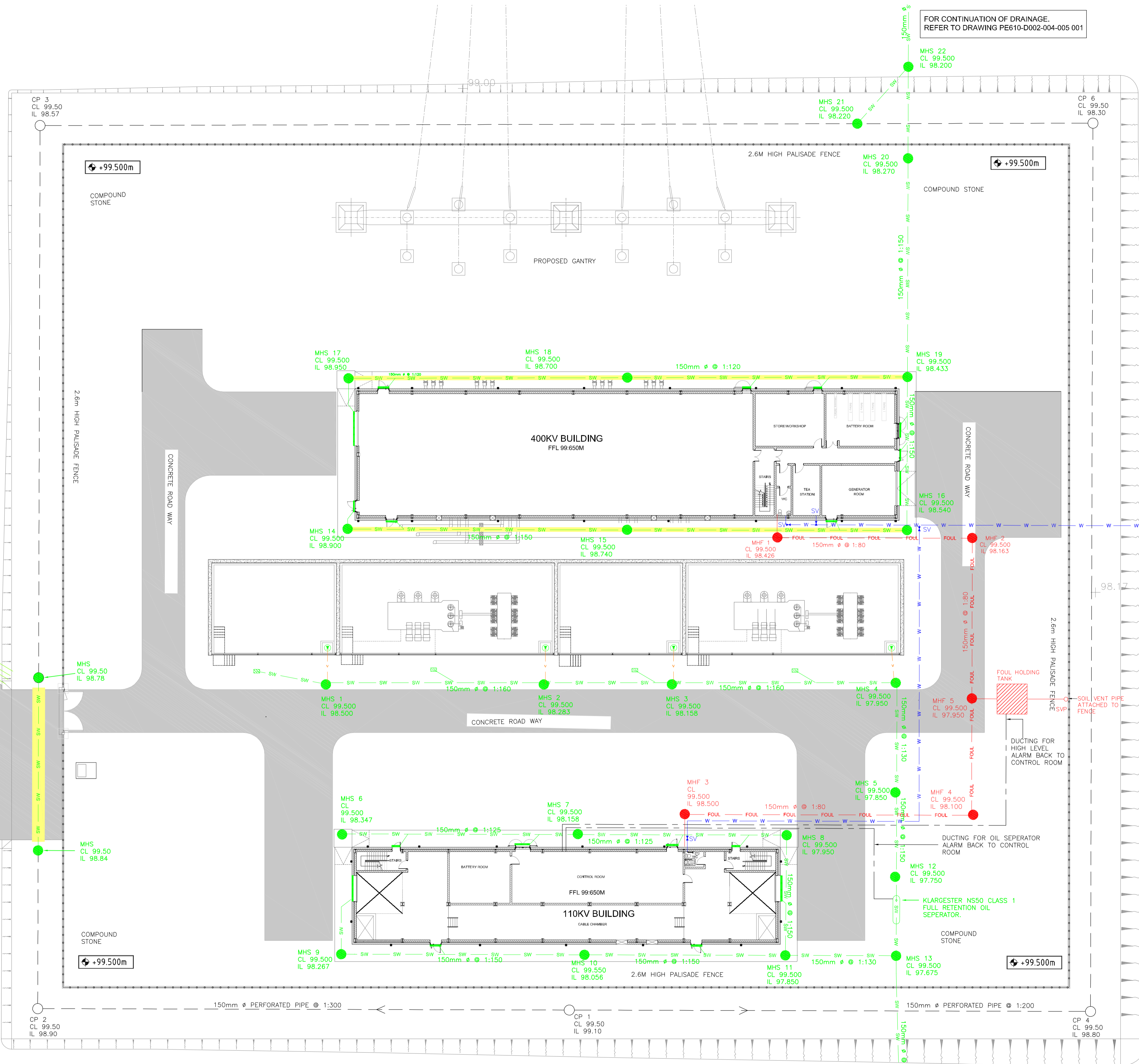
COMPOUND DRAINAGE LAYOUT SCALE 1:250
